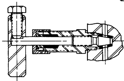
MODEL 55B BONNET ASSEMBLY WITH TEFLON PACKING
