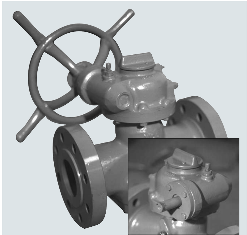
Spur gearing for standard valves. Handwheel pinion rotates upon upper end of plug shank.
