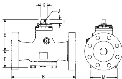
ASME Class 300 – Figure 2545
