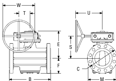
ASME Class 300 – Figure 2549
