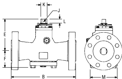
ASME Class 150 – Figure 2445
