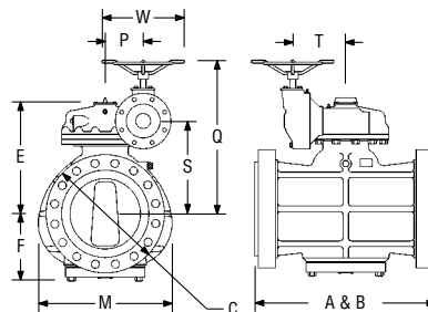
Fig. 6049, Size 16 (worm or bevel gearing)
