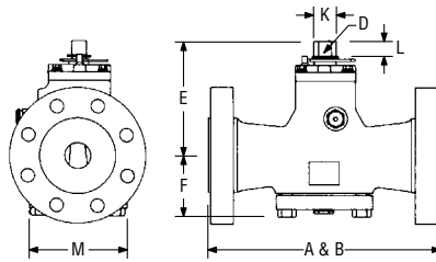
Fig. 76305, Sizes 2½ to 4½ Fig. 76505, Sizes 2½ to 4½
