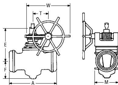
Figure 4189½, Sizes 6, 8 and 12
